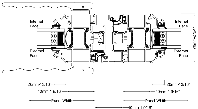
Section 8: Swing panel and slave panel with closing rebates
