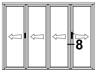
Section 8: Swing panel and slave panel with closing rebates
