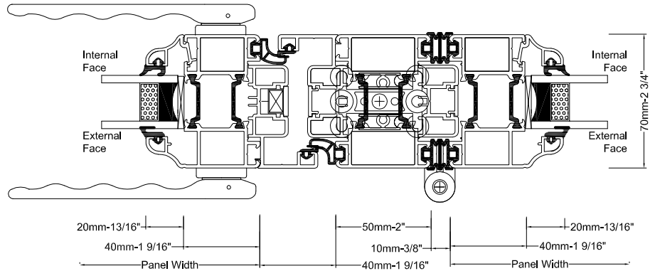
Section 10: Sliding mullion and swing panel with closing rebates and roller assembly
