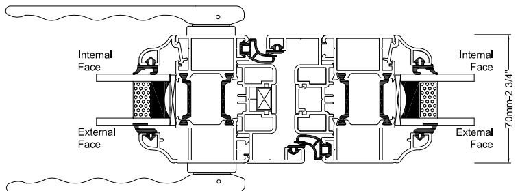
Section 8: Swing panel and slave panel with closing rebates
