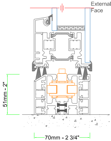
Raised Track
