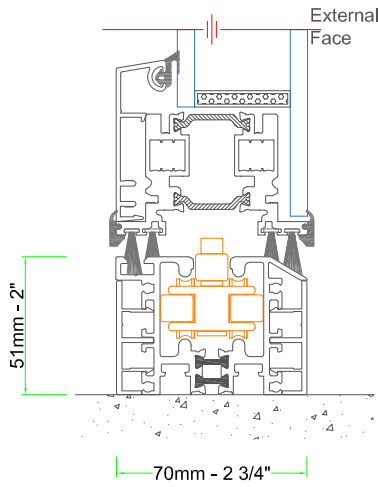
Raised Track
