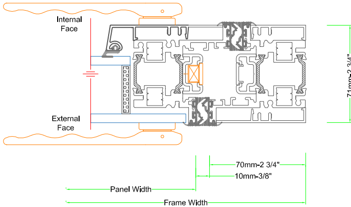
Section 7: Swing panel and jamb with closing rebates
