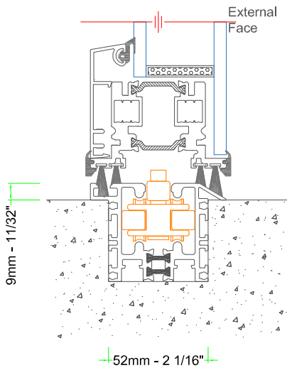
Flush Track
