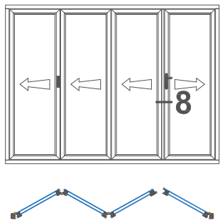
Section 8: Swing panel and slave panel with closing rebates
