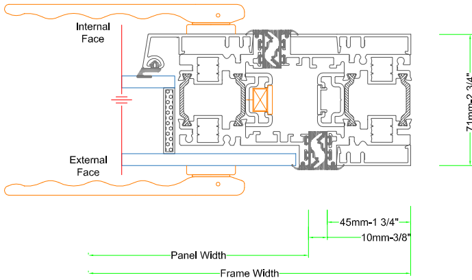
Section 7: Swing panel and jamb with closing rebates
