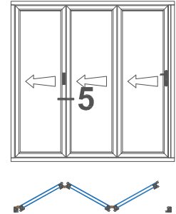
Section 5: Locking folding panels, with Flat Handle
