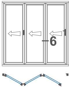
Section 6: Non-locking folding panels and roller assembly
