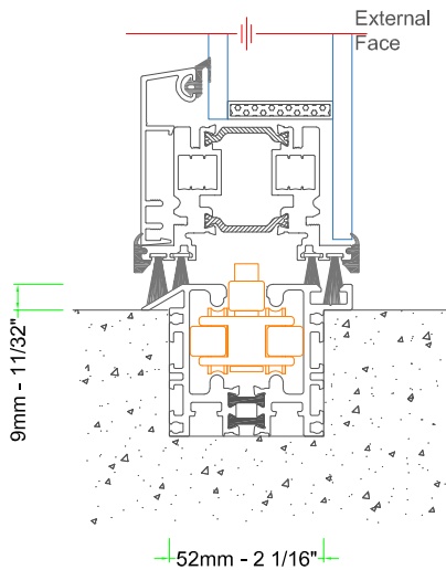
Flush Track
