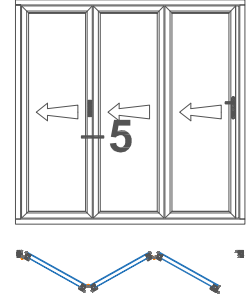
Section 5: Locking folding panels, with Flat Handle
