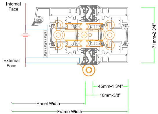
Section 4: Jamb with Roller Assembly
